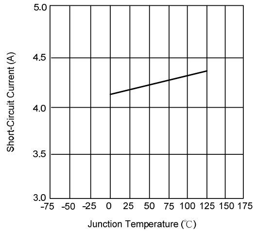
Figure 8. Short-Circuit Current vs. Temperature
